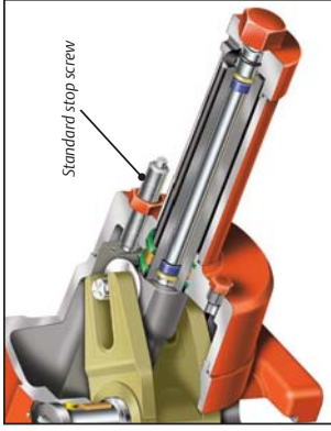
M11 Hydraulic Override Configuration
